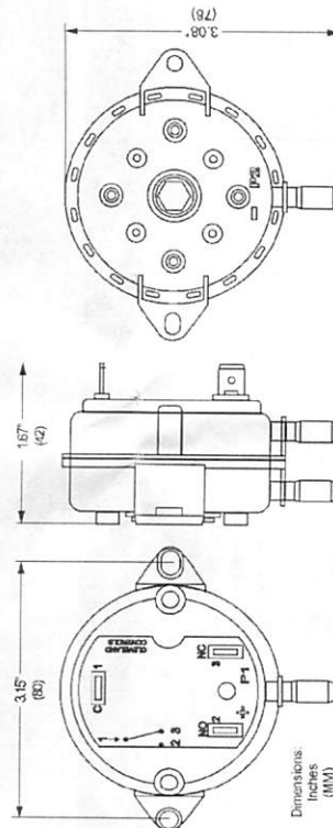
FIGURE 6: DIMENSIONS OF NS2 SWITCH WITH INTEGRAL CONNECTORS AND MOUNTING FEET. THE STANDARD CONNECTORS ACCEPT FLEXIBLE TUBING.
